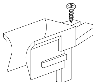
NYL-370 - Guia da persiana de enrolar
