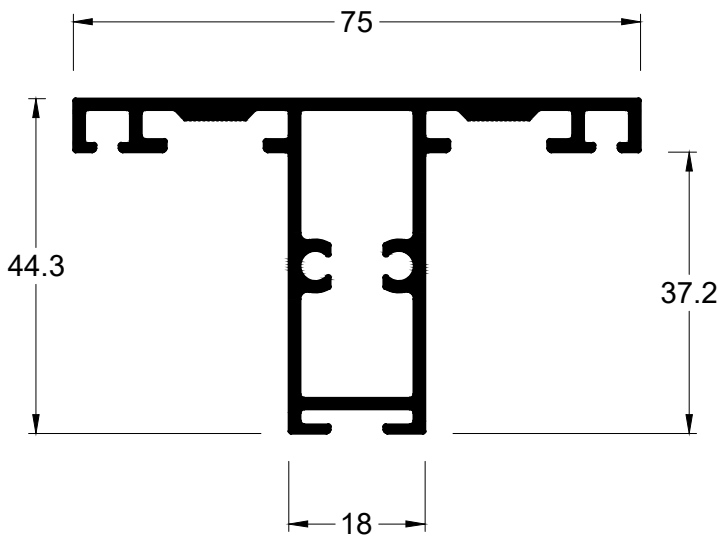
FC-231 1,053 kg/m Coluna
