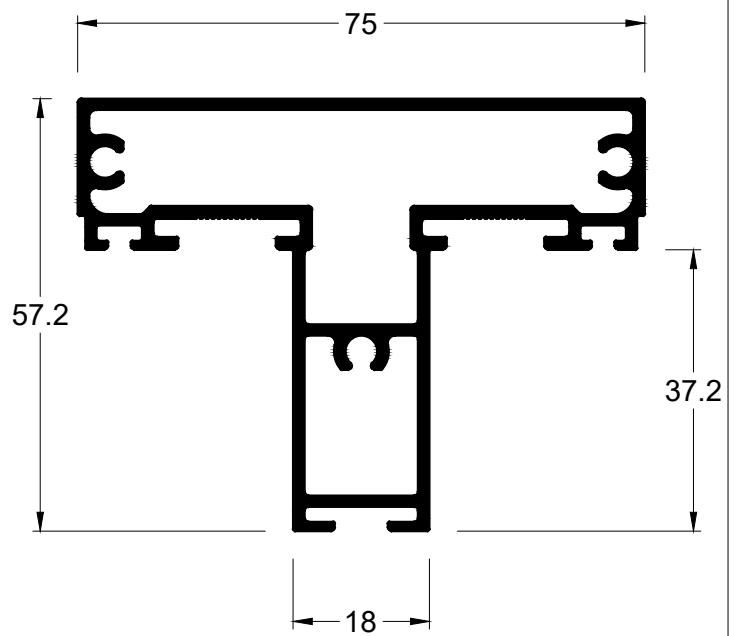
FC-517 1,441 kg/m Coluna
